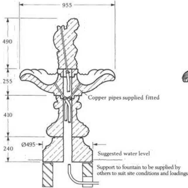
SECTION SCALE 1:20 Core Ø 75mm.
